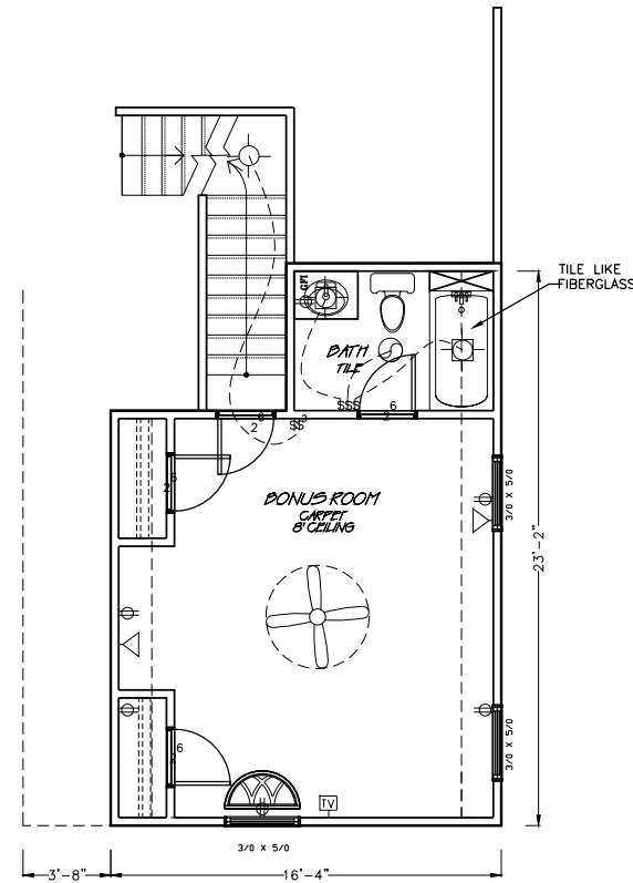
2 BONUS FLOOR PLAN 1/4" = 1'-0"
