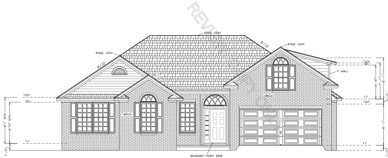
1 FRONT 1/4" = 1'-0"
